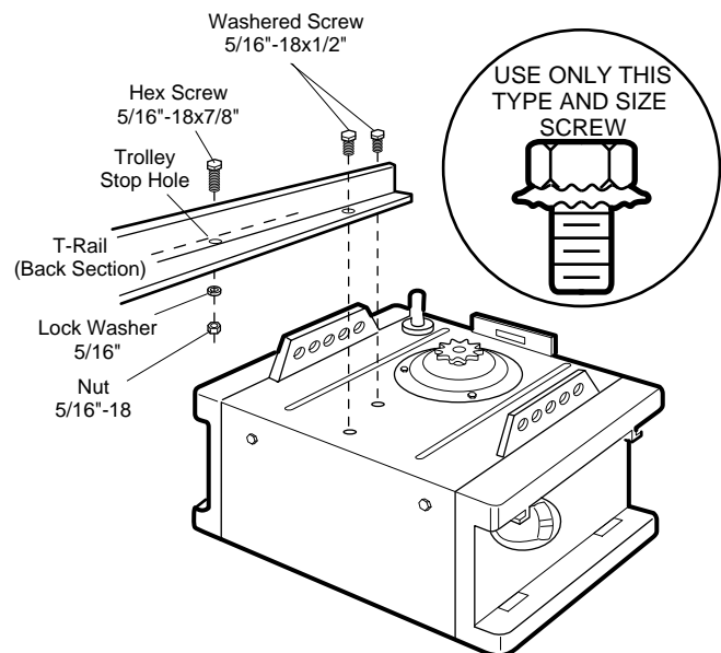
Lock Washer 5/16"
