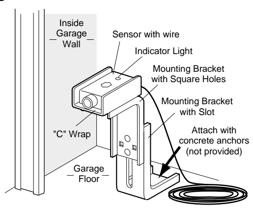
Figure 5 Alternate Floor Mount
