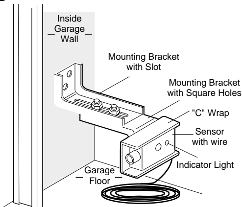
Figure 4 Alternate Wall Mount
