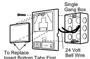
Figure 2 PRE-WIRED INSTALLATION
