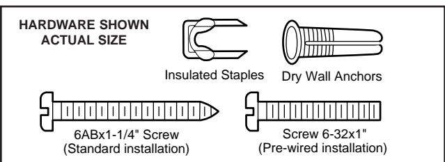
Figure 1 STANDARD INSTALLATION
