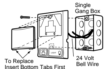
Figure 2 PRE-WIRED INSTALLATION
